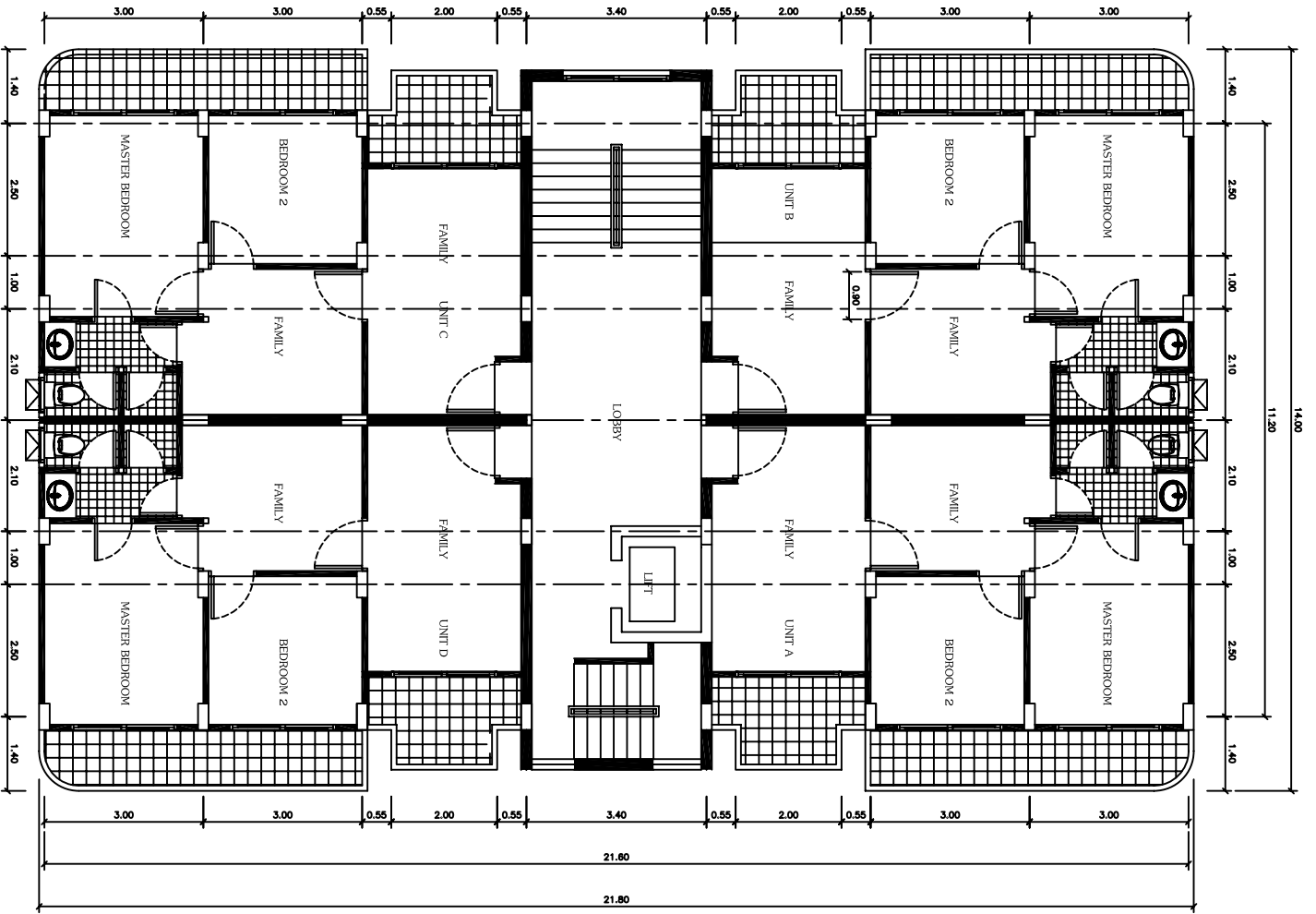
FLOOR PLAN 1:75
